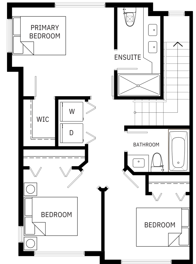
THIRD FLOOR
