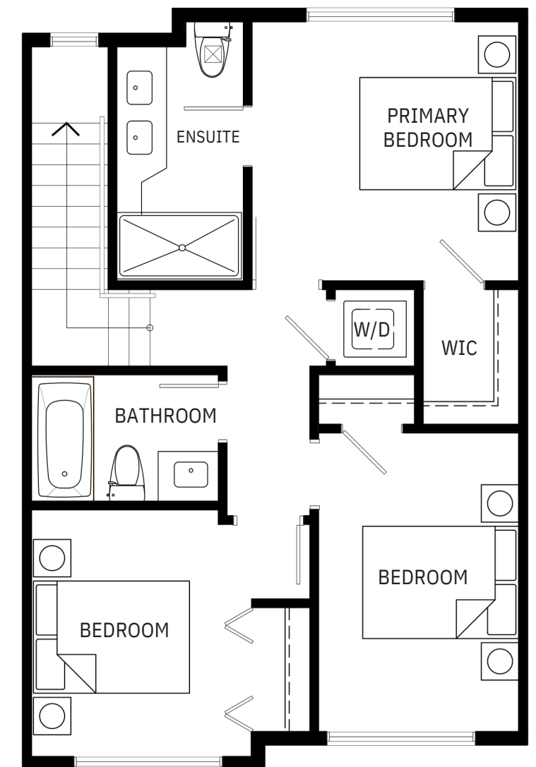
THIRD FLOOR
