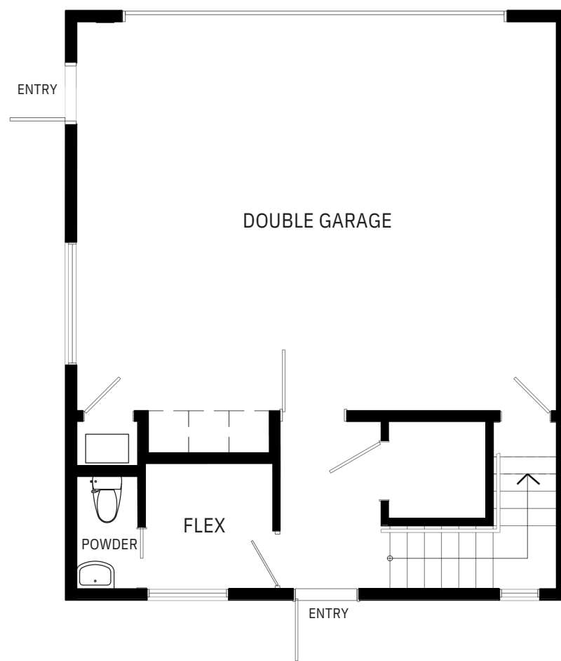
MAIN FLOOR
